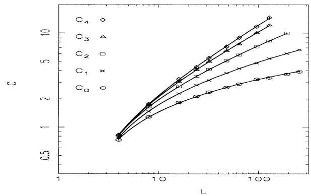
FIG. 2. Specific heat C as a function of \ln L for five critical models C_0, \dots, C_4 , of the AAT. Note that C_0 is an anisotropic decoupled Ising model and C_4 is an anisotropic four-state Potts model. The curves are fits to (27), yielding estimates for \frac{\alpha}{\nu} which are listed in Table I.
